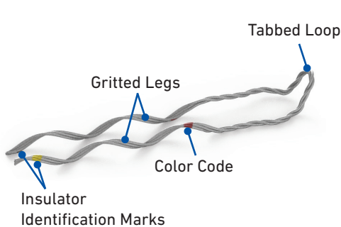
Tabbed Style Double Support Tie
