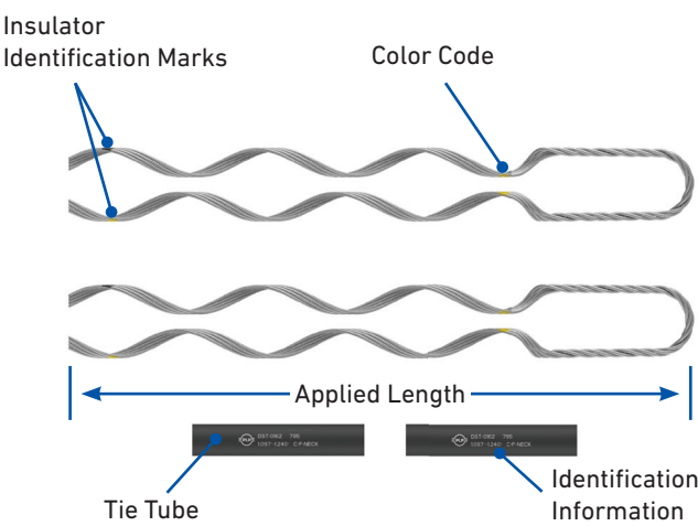
Figure 2: Hairpin Style Tie Assembly
